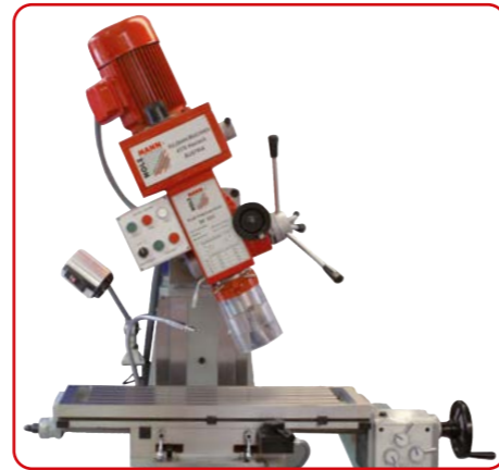
schwenkbarer Fräskopf pivotable milling head
